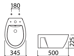
131455 bidé suspenso com furação para tampo wall hung bidet w/ holes f/ cover bidet suspendu a/ trous p/ abattant
